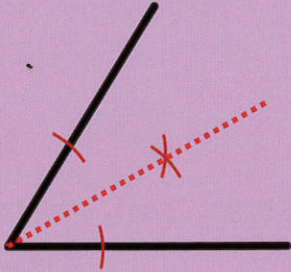
Angle Bisector
