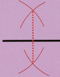
Perpendicular Bisector
